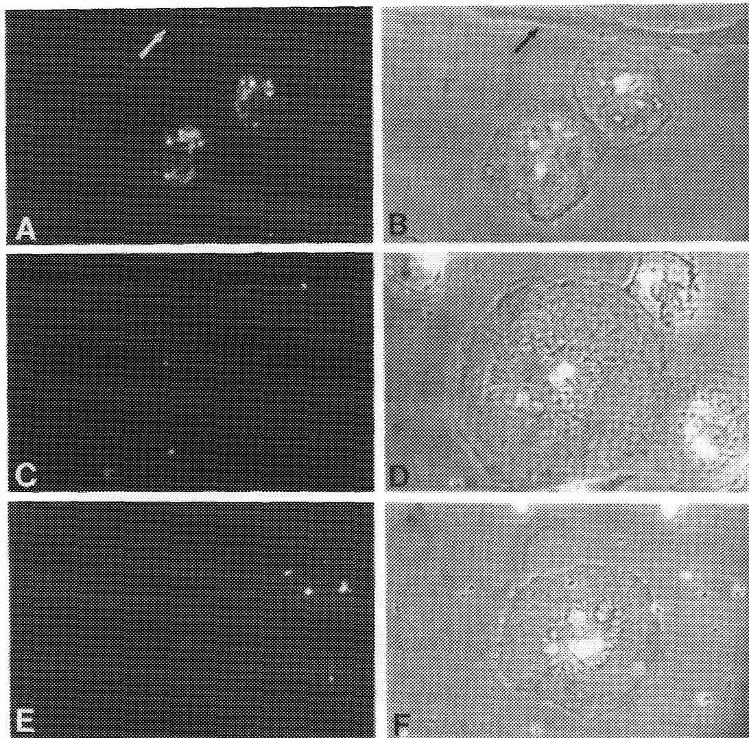
Figure 6. Fluorescent and phase contrast images of osteoclasts. (A) Osteoclasts treated with 2\mu\text{M} 17\beta\text{-E}_2\text{-BSA-FITC} for 40 minutes; fluorescence was centrally located and the adjacent fibroblast (arrow) did not stain. (B) Phase contrast of A; arrow points to fibroblast. (C) Osteoclast incubated with 2\mu\text{M} 17\beta\text{-E}_2\text{-BSA-FITC} and 1\mu\text{M} 17\beta\text{-estradiol} to block staining resulted in substantially less fluorescence. (D) Phase contrast of C. (E) Osteoclast incubated in 0.625\mu\text{M} BSA-FITC for 40 minutes as the control. Note that there were barely detectable amounts of fluorescence. (F) Phase contrast of E (460x).
